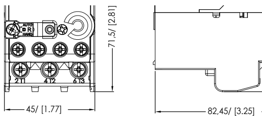
WR17-1D
