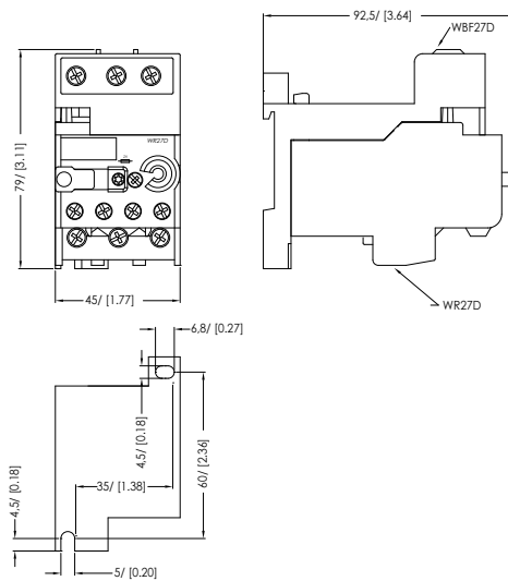
WR27 + WBF27
