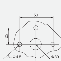
Installation size of operation outside board handle
