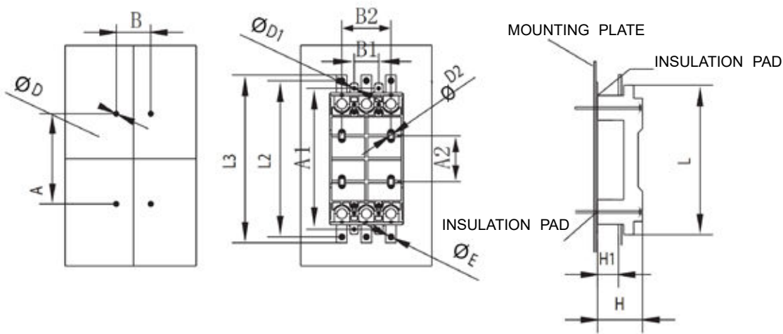
Rear connection & overall (mm)
