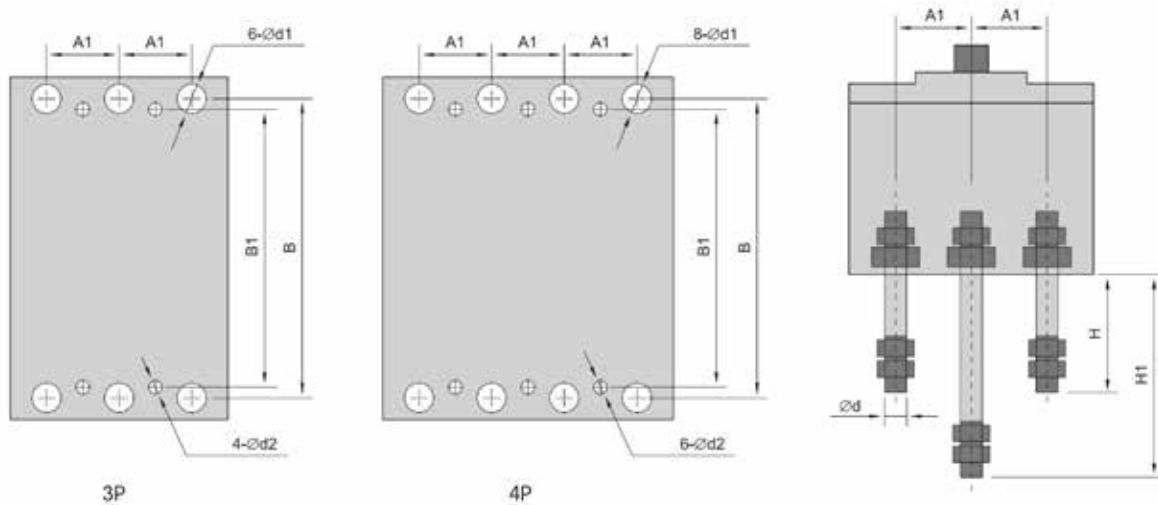
Plug in connection &amp; overall (mm)
