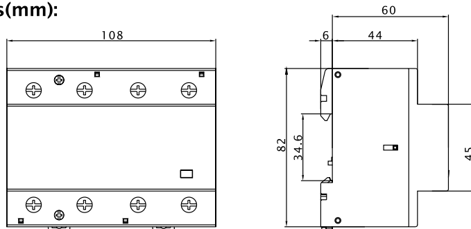
Dimensions(mm):
