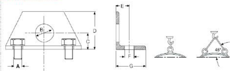
Lifting reinforcements
