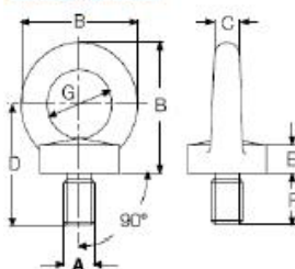
Lifting eyebolts
