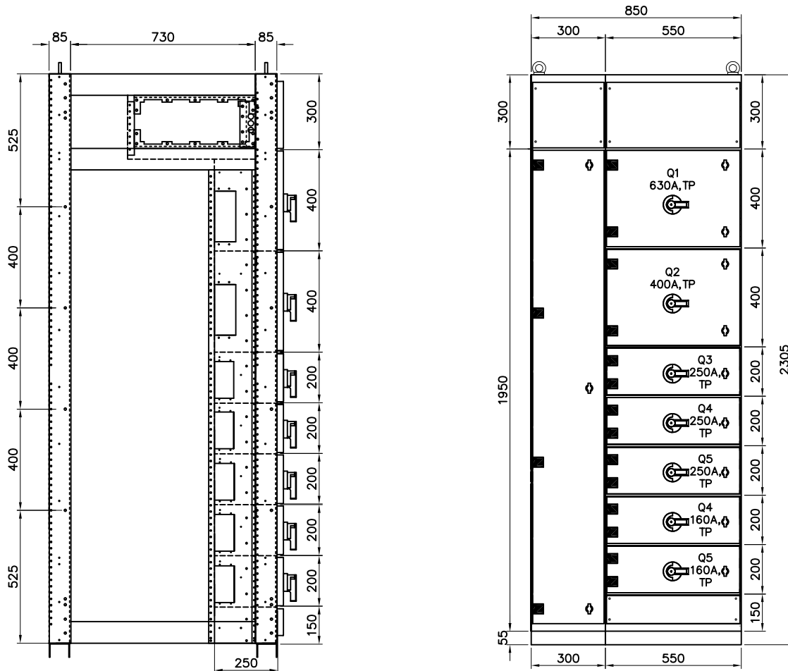
FRONT VIEW
